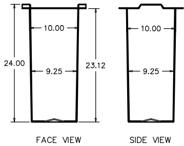
FACE VIEW
